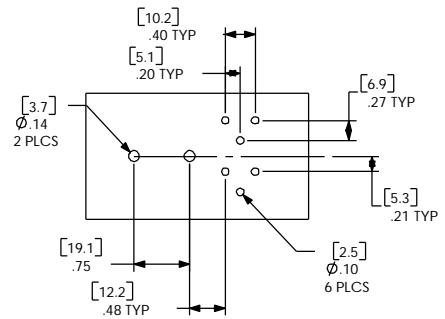
SUGGESTED PC BOARD HOLE LAYOUT
