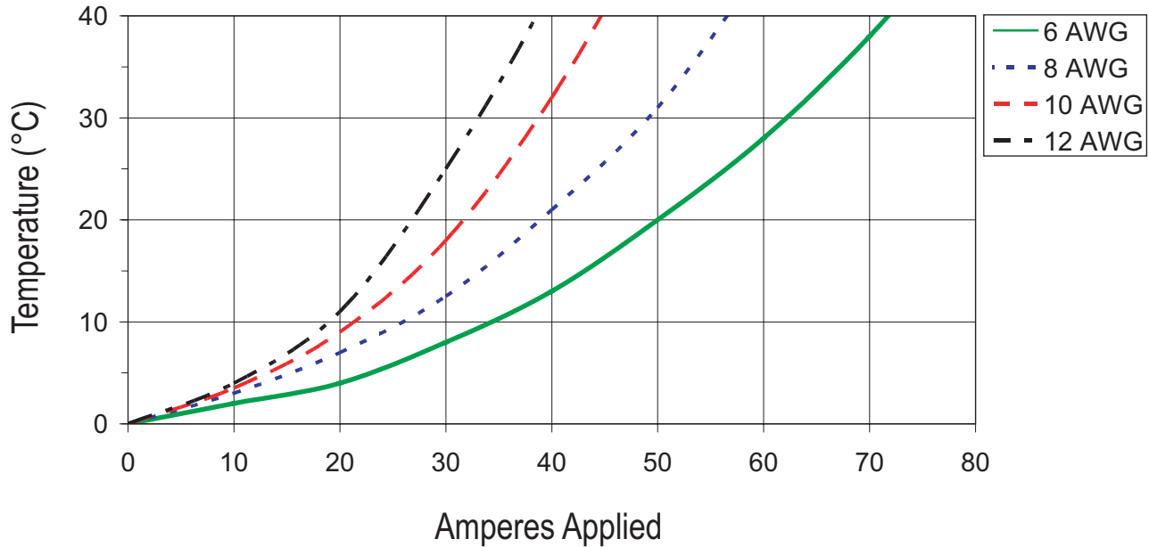
SBS50 Temperature Rise at Constant Current
